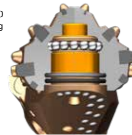
Charger™ RR440/450 sealed journal bearing
