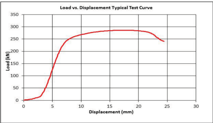
Load tested in compression over 70mm hole with 24mm self aligning ball washer.
