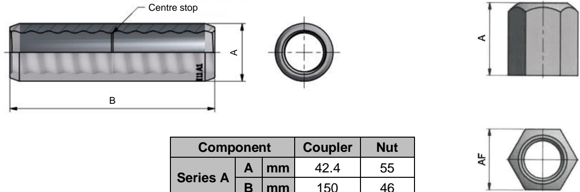
Figure 1: Coupler, Nut
